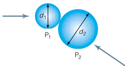
Figure 19.8 If the gas particles involved in the collision are of different types, then two different masses and diameters enter the equation for collision frequencies.
