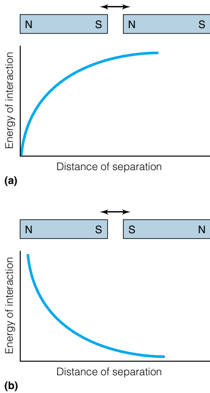
Figure 16.5 Interactions can be (a) attractive or (b) repulsive. Attractive interactions contribute to a lowering of the overall energy, whereas repulsive interactions contribute to an increase in the overall energy. The interactions of the two bar magnets shown mimic the interactions of magnetic fields and magnetic dipoles.
