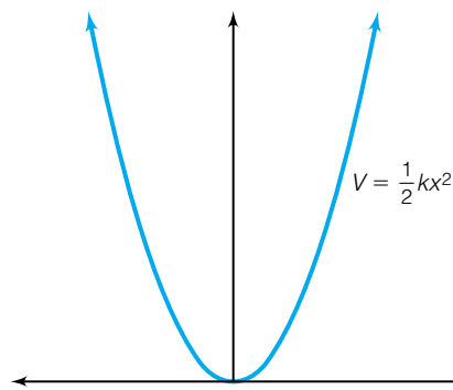
Figure 11.1 A plot of the potential energy diagram V(x) = \frac{1}{2}kx^2 for an ideal harmonic oscillator.
