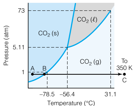
Figure 6.11 An illustration of the isobaric change for \text{CO}_2 specified in Example 6.10a. Compare this to Figure 6.12.
