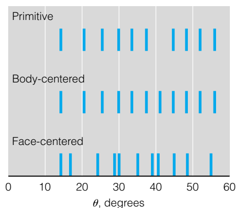
Figure 21.24 The pattern of diffracted X rays is characteristic of the type of unit cell a crystal has. Here, the patterns that the three cubic Bravais lattices cause on the X-ray diffraction is illustrated. For all three, we are assuming a unit cell parameter of 3.084 \text{ \AA} and an X-ray wavelength of 1.542 \text{ \AA} . Compare these patterns with the films in Figure 21.23: can you detect any correspondences between these two figures?
