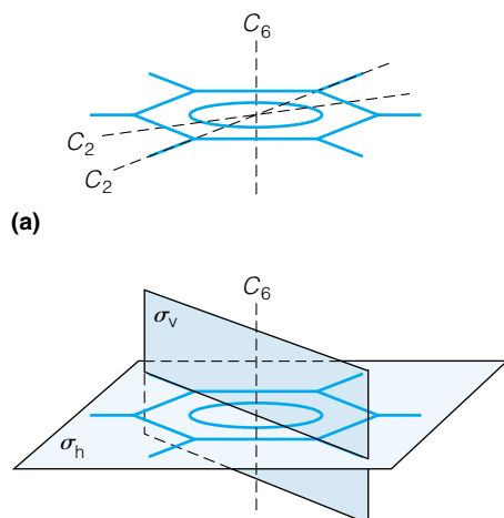
Figure 13.6 (a) The benzene molecule has one sixfold principal axis of symmetry, C_6 . It also has several C_2 axes of symmetry perpendicular to the principal axis, in the plane of the molecule. Only two are shown. Can you find all of the other axes of symmetry? (b) Reflection planes are vertical planes if they contain the principal axis of symmetry, and horizontal planes if they are perpendicular to the principal axis. There are also dihedral planes, which are vertical planes that bisect two intersecting C_2 axes of symmetry. In the benzene molecule, the vertical planes are actually dihedral planes.
