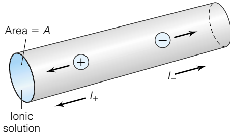
Figure 8.10 Ionic current travels in two directions, and is measured in terms of how many ions pass through some cross-sectional area A per unit time.
